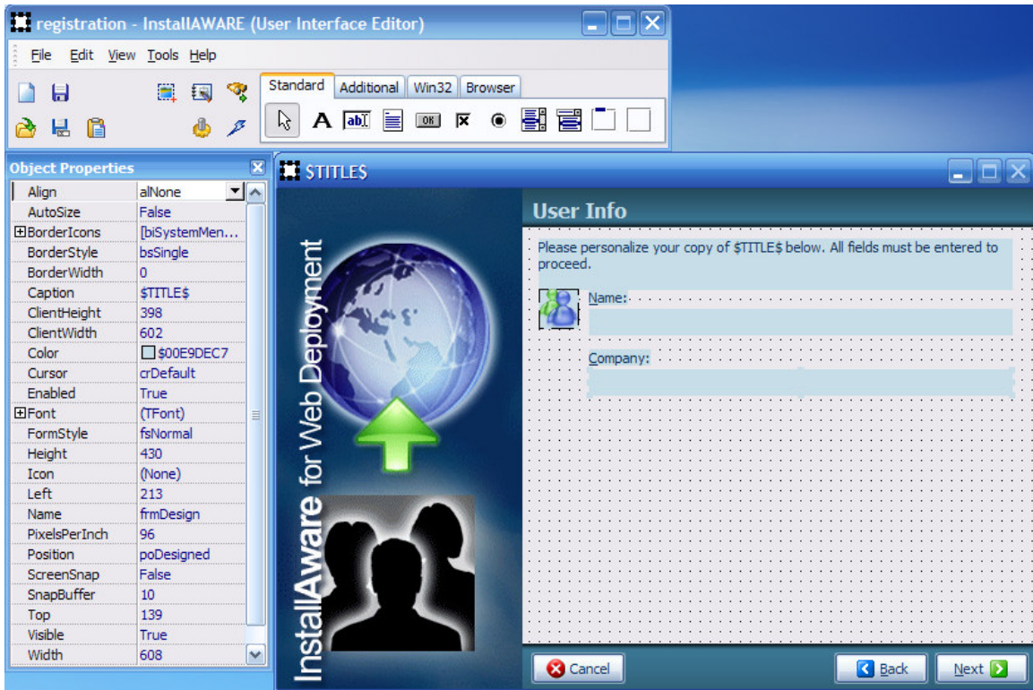
Figure 3 The Dialog Editor
