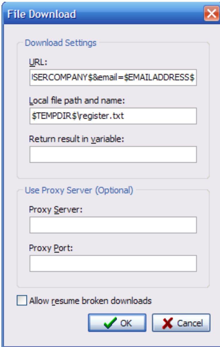
Figure 7 The File Download Plug-In
