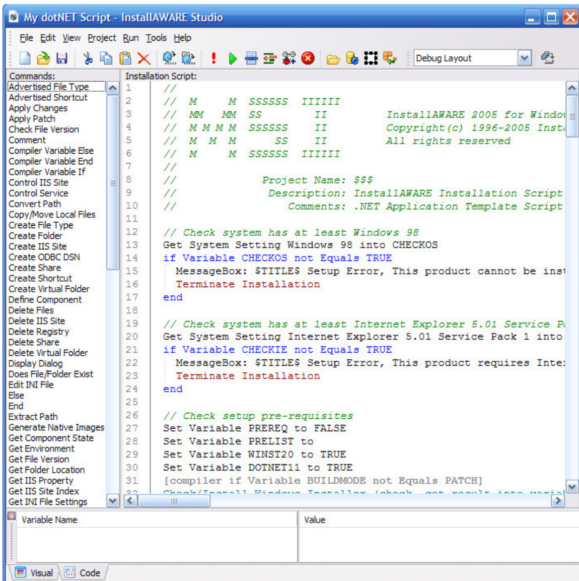
Figure 2 The InstallAware Script
