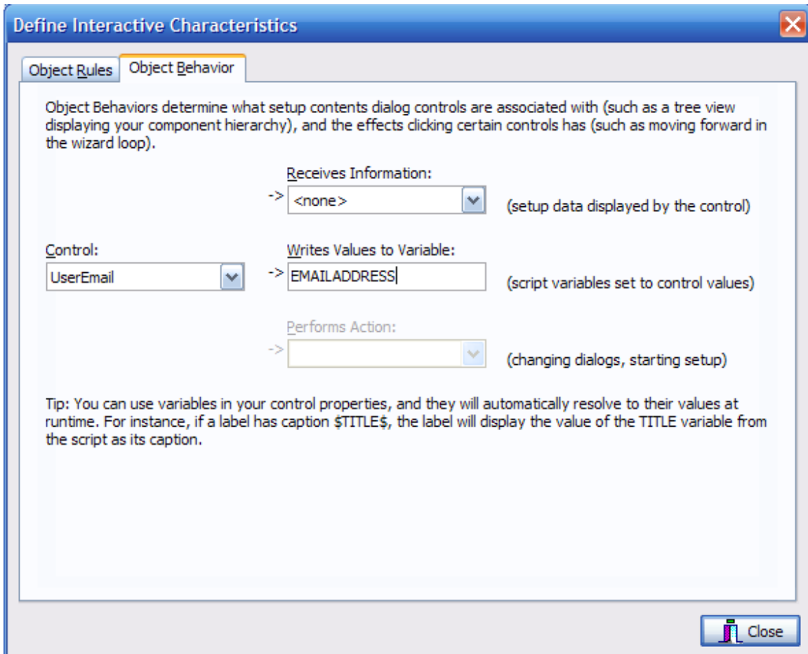
Figure 4 Assigning Script Variables to Dialog Controls
